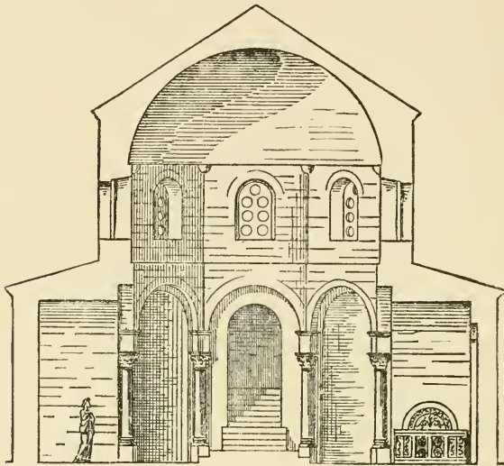
Fig. 139.—Vertical section of the baptistery in Albegna, Italy.
